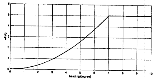
Fig.A2 Workload w_{hdg} for Straight Flight
