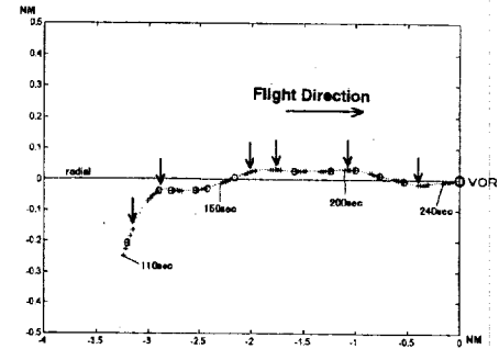
b) Flight History
