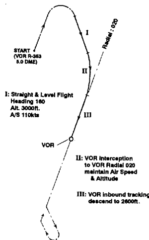
Fig.3 Flight Scenario
