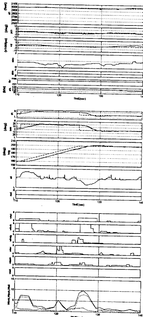
Fig.4 Time Histories of Flight Parameters and Workload (Horizontal Turning Flight, Pilot A)
