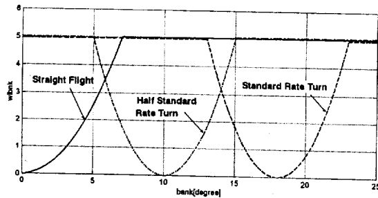
Fig.A1 Workload w_{bnk}
